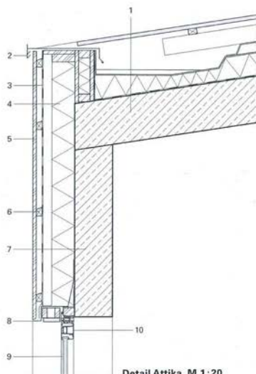
Detail Attika, M 1:20
